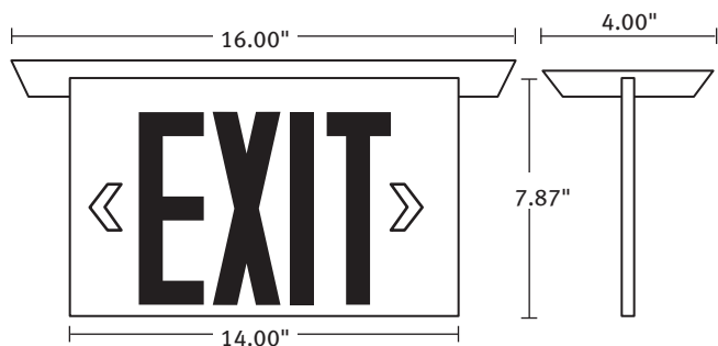
SPECIAL RECESSED MOUNT
