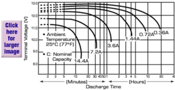
Discharge Time vs. Terminal Voltage
