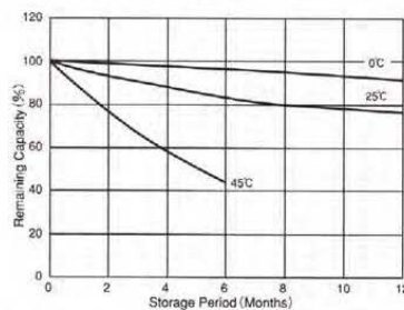
Self-discharge Characteristics
