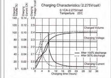
Charging Characteristics(2.275V/cell)
