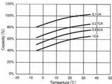
Temperature and Discharge Capacity
