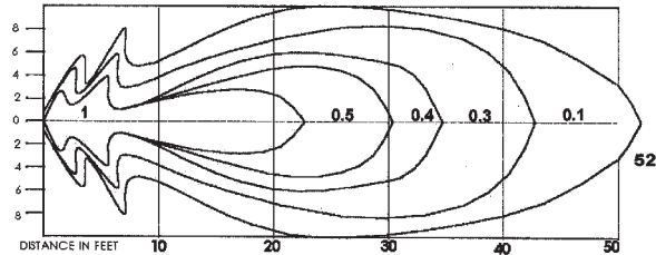
Lamp Photometrics 6 Volt 5.0 Watt MR-16 Halogen Lamp
