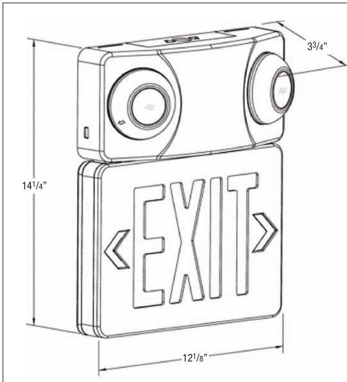
Combination exit and emergency light
