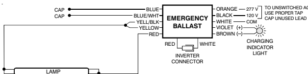
FIG 1a ONE (1) 32 W T8 LAMP WITHOUT AC BALLAST
