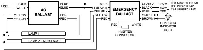
FIG 3a TWO (2) LAMP RAPID START BALLAST
