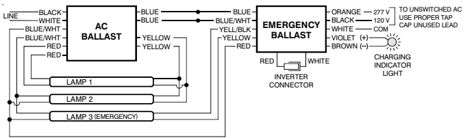
FIG 15a THREE (3) LAMP RAPID START BALLAST
