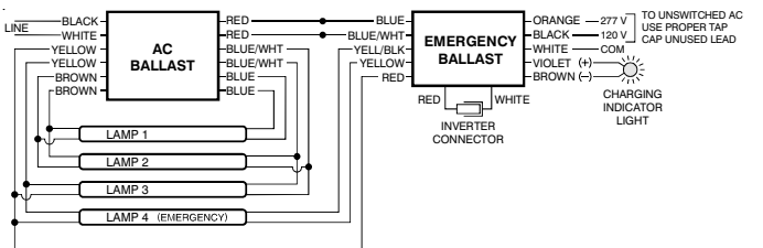
FIG 51a FOUR (4) LAMP RAPID START BALLAST
