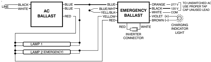
FIG 36a TWO (2) LAMP INSTANT START BALLAST
