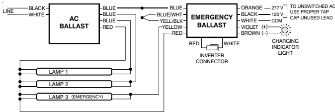
FIG 7a THREE (3) LAMP INSTANT START BALLAST
