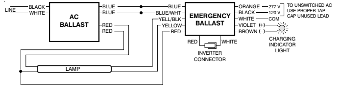
FIG 2a ONE (1) LAMP RAPID START BALLAST
