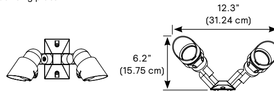
double CEF with rectangular mounting plate
