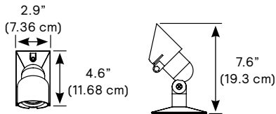
single CEF with rectangular mounting plate
