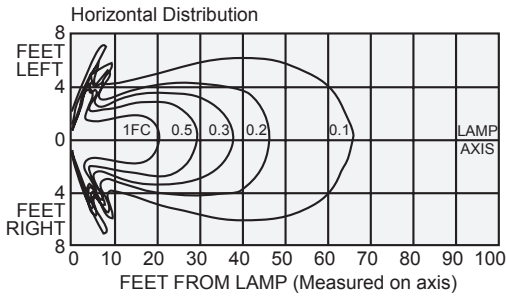
6V, 5W Halogen MR16 Lamp, MR16 Head
