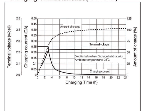
Charging Characteristics (2.23V/cell)
