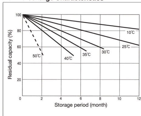
Self-discharge Characteristics
