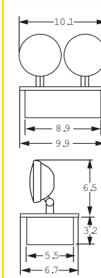
Round Heads Suffix "-R"
