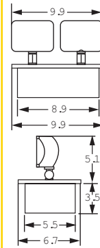
Rectangular Heads Suffix "-PH"
