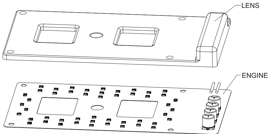
Exploded View
