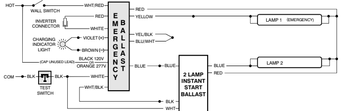
FIG 107A TWO (2) LAMP INSTANT START BALLAST FOR 4-PIN LONG COMPACT
