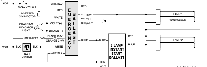
FIG 107A TWO (2) LAMP INSTANT START BALLAST FOR 4-PIN LONG COMPACT
