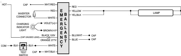
FIG 109 ONE (1) 14 W - 55 W LAMP WITHOUT AC BALLAST
