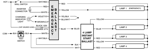
FIG 123 FOUR (4) LAMP INSTANT START BALLAST
