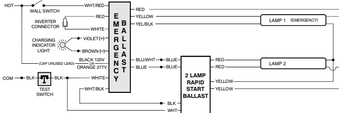
FIG 107 TWO (2) LAMP RAPID START BALLAST FOR 4-PIN LONG COMPACT
