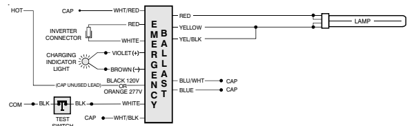
FIG 109a ONE (1) 36 W - 55 W LAMP WITHOUT AC BALLAST
