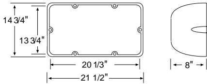
CPS-4X Cover Dimensions
